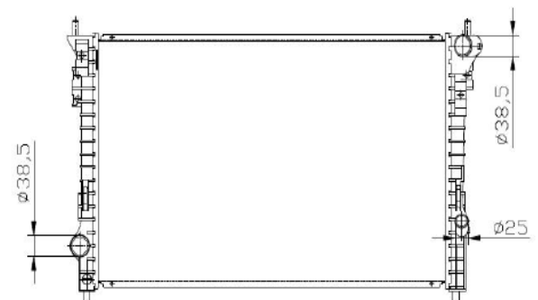
FORD EDGE (M/T) 730 X 438 X 26mm (A/P) OE Ref.: 7T4Z8005B DPI: 2937
