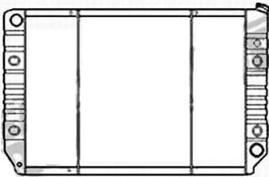
CHEVROLET GMC TRUCK (A/T) 870 X 520 X 3R-C/B OE Ref.:----- DPI 1218
