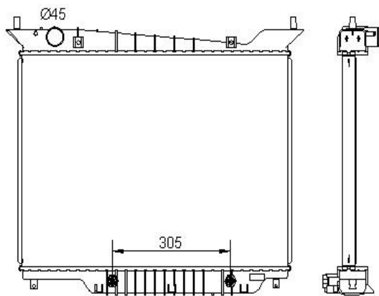
Expedition (A/T) 506 X 688 X 36mm (A/P) OE Ref.: 2LIZ8005DD/9DF DPI: 2609
