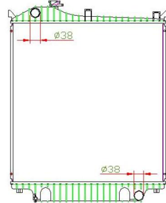
Explorer 2006 (M/T) 610 X 578 X 32mm (A/P) OE Ref.: 6L2Z8005AA DPI: 2816
