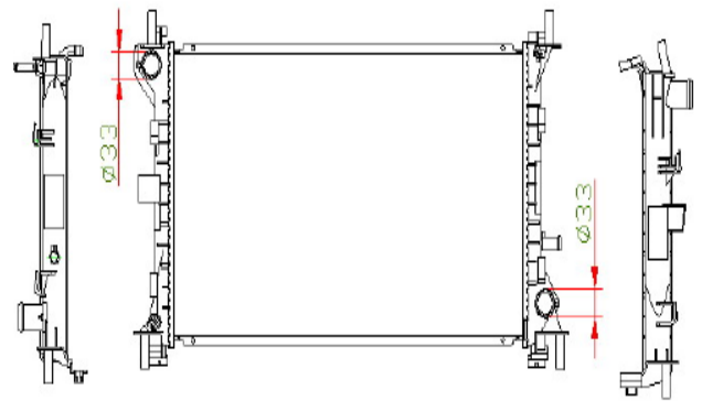
FOCUS 2000-2001 (M/T) 600 X 348 X 26mm (A/P) OE Ref.:YS4Z8005AA /1061191 DPI: 2297
