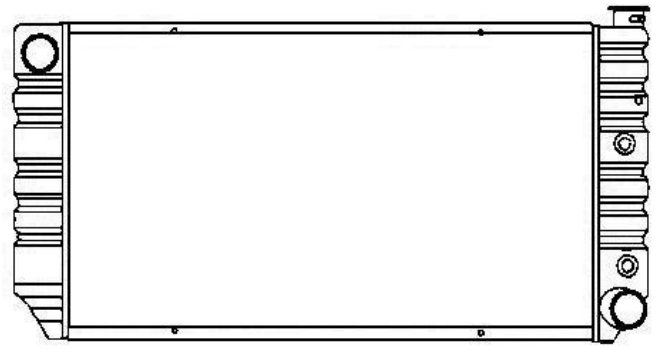
CHEVROLET GMC TRUCK (A/T) 870 X 460 X 3R-C/B OE Ref.:----- DPI 1364
