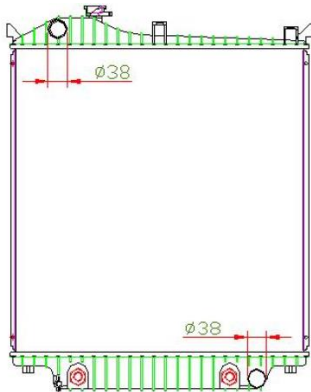
Explorer 2006 (A/T) 610 X 578 X 32mm (A/P) OE Ref.: 6L2Z8005AA DPI: 2816
