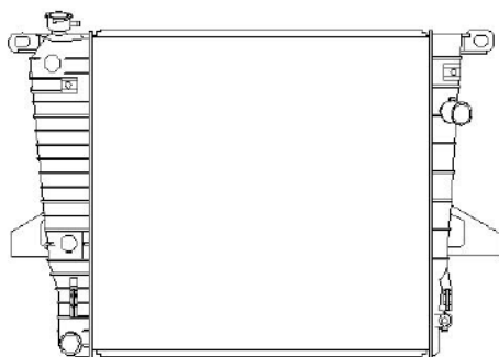
Explorer 1997-2001 (A/T) 510 X 538 X 48mm (A/P) OE Ref.: F57H8005NB DPI: 1728
